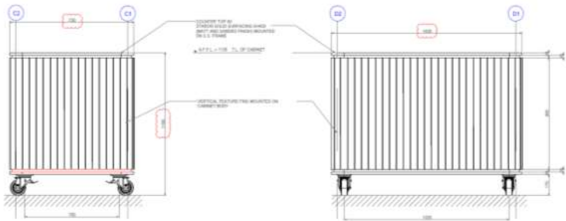
1 SIDE ELEVATION 1:16
